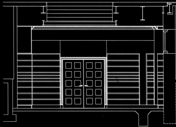
2 WEST ELEVATION 1/8" = 1'-0"
