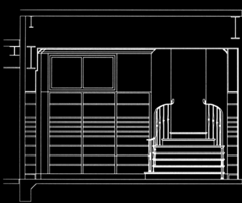
1 NORTH ELEVATION 1/8" = 1'-0"
