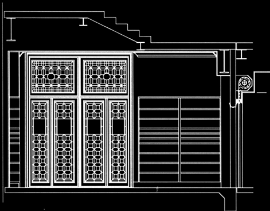
3 SOUTH ELEVATION 1/8" = 1'-0"
