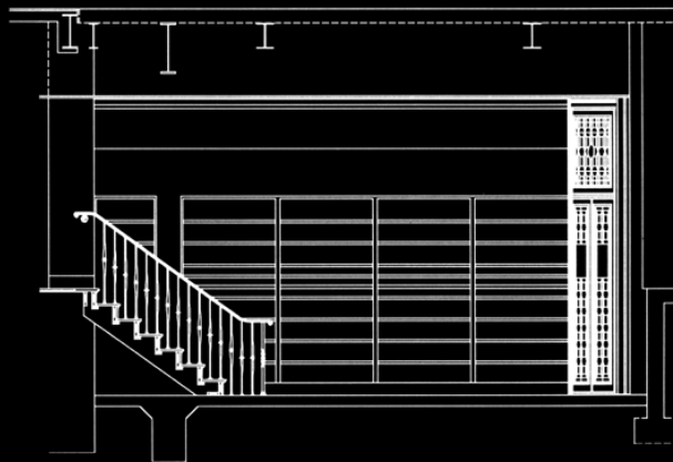
4 EAST ELEVATION 1/8" = 1'-0"
